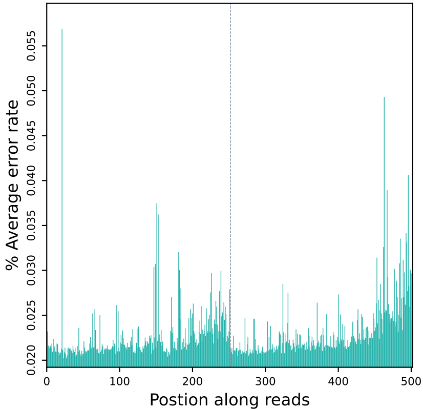
Error rate distribution along reads (R10814)
